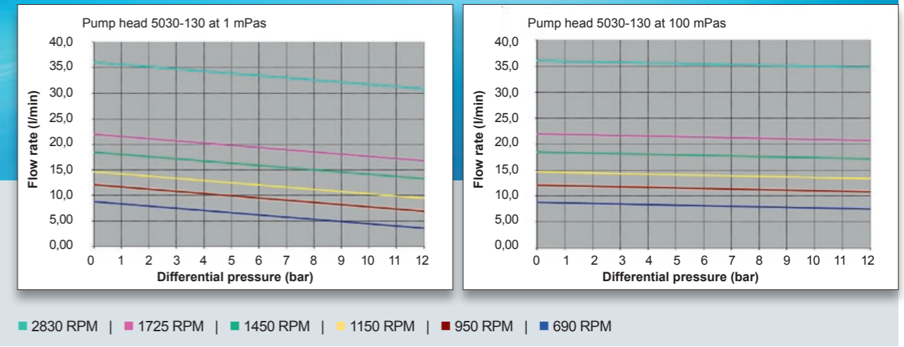
Performance curves of pump size 5030-210
