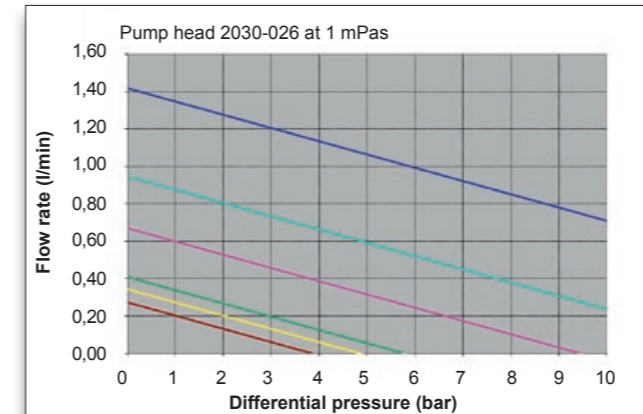
Performance curves of pump size 2030-026
